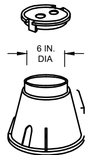
6 IN. DIA TURF BOX PLEASE REFER TO W-6 WHEN 4 IN. PVC SLEEVE IS EXPOSED TO TRAFFIC OR IS IN THE SIDEWALK.
