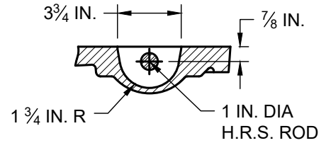
PICKBAR DETAIL
