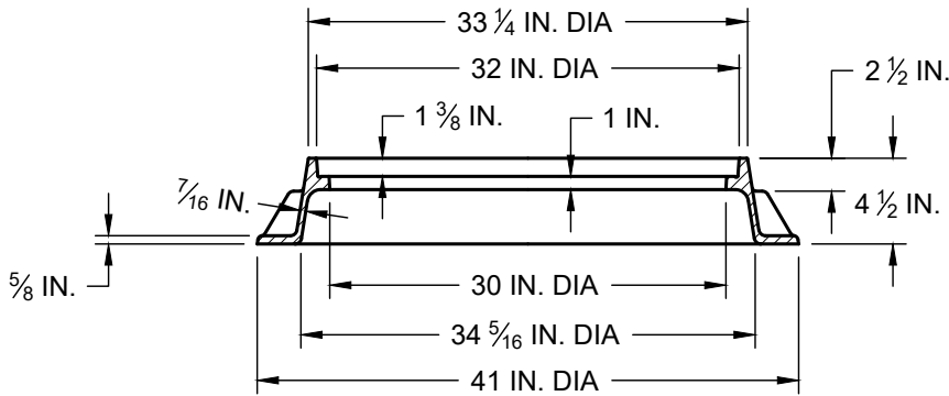
FRAME SECTION
