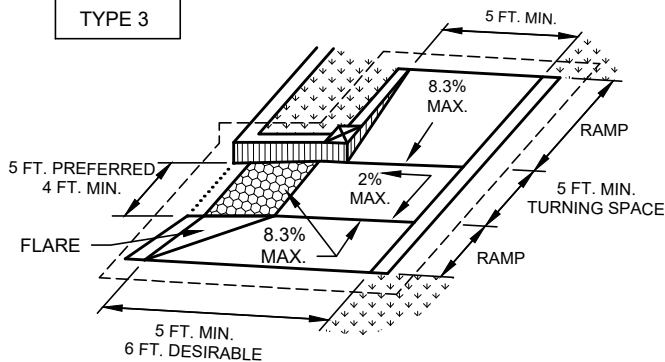
COMBINATION CURB RAMPS
