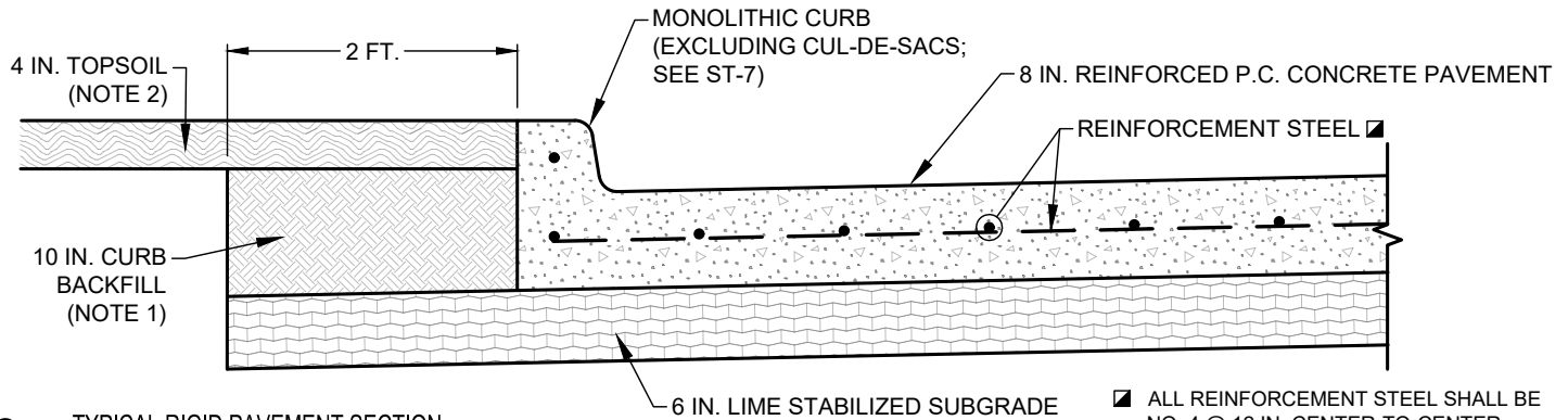
IC2 (R) TYPICAL RIGID PAVEMENT SECTION: INDUSTRIAL COLLECTOR STREET (20 < P.I. < 40)
