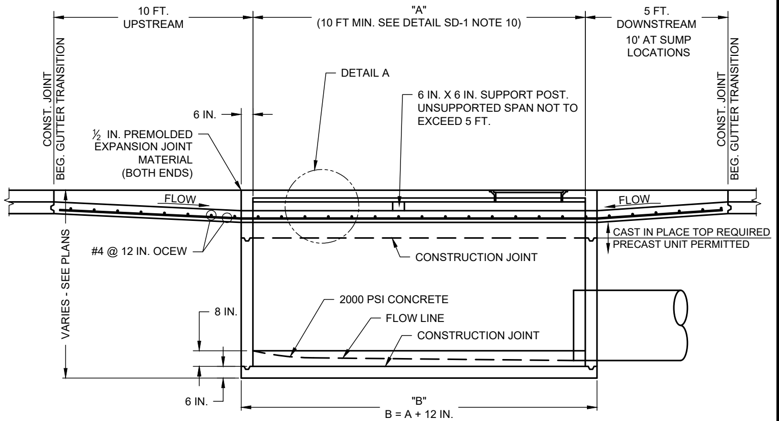
FRONT SECTION VIEW
