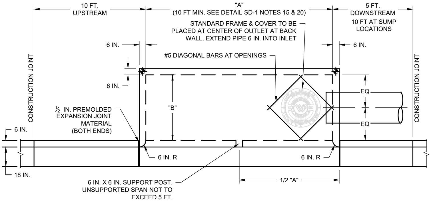
PLAN VIEW
