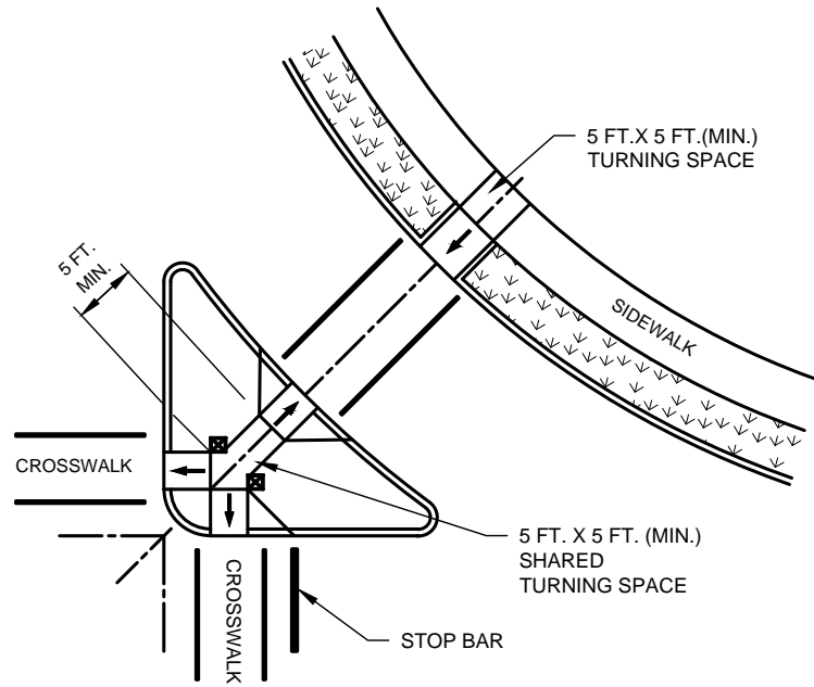
AT INTERSECTION WITH FREE RIGHT TURN & ISLAND
