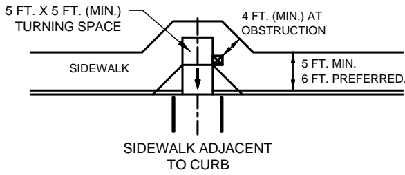
MID-BLOCK PLACEMENT PERPENDICULAR RAMPS
