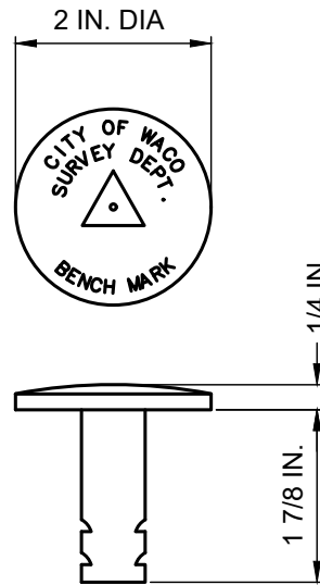
BENCHMARK DETAIL NTS
